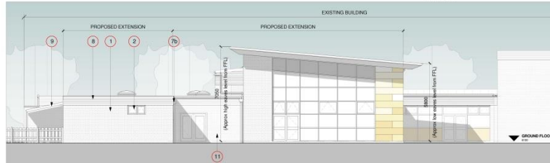
Proposed Elevation 3b_East Elevation 1 : 100
