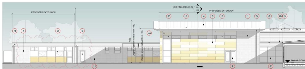
Proposed Elevation 1_North Elevation 1 : 100
