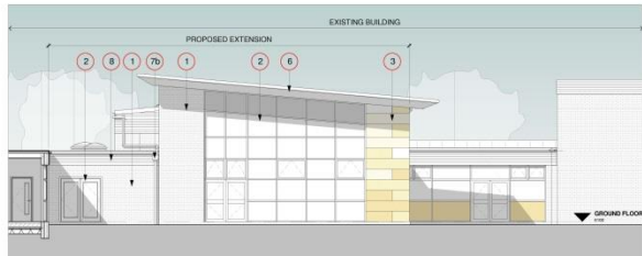
Proposed Elevation 3a_East Elevation 1 : 100
